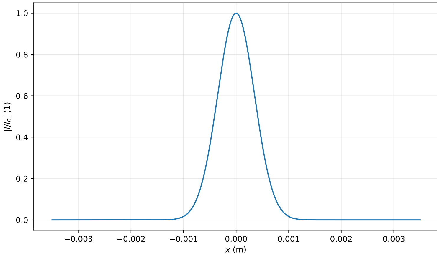
Intensity profile I(x, y = 0, z = 0.080m)/I_0 , P_{in}=0.2P_{cr} , artificial time
